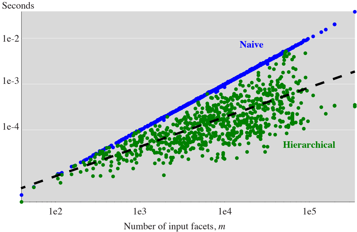
Figure 8.11: Hierarchical evaluation performs asymptotically better than the naive implementation on a large set of different meshes. Naive (blue) fits neatly to m^{1.00} , hierarchical (green) fits in least squares sense to m^{0.55} (black line).
