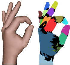
Figure 2: One of 27 hand poses with core bone triangles for 17 estimated bones ( \epsilon = 0.05 ). Although our method can skin mesh sequences with pre-existing skeletons (§5), its strength lies in optimizing non-hierarchical bone transforms for each frame (§4), and avoiding pose space interpolation of progressive skin corrections (§6).
